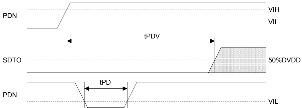
Figure 7. Power Down & Reset Timing
