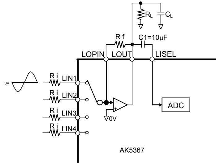
Figure 2. Pre-Amp Circuit
