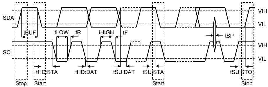
Figure 6. I 2 C Bus mode Timing
