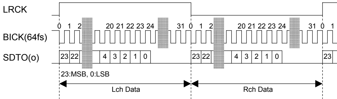
Figure 8. Mode 0 Timing
