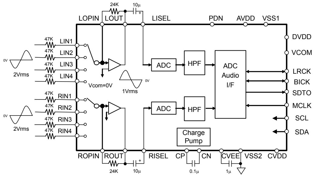
Figure 1. AK5367 Block Diagram
