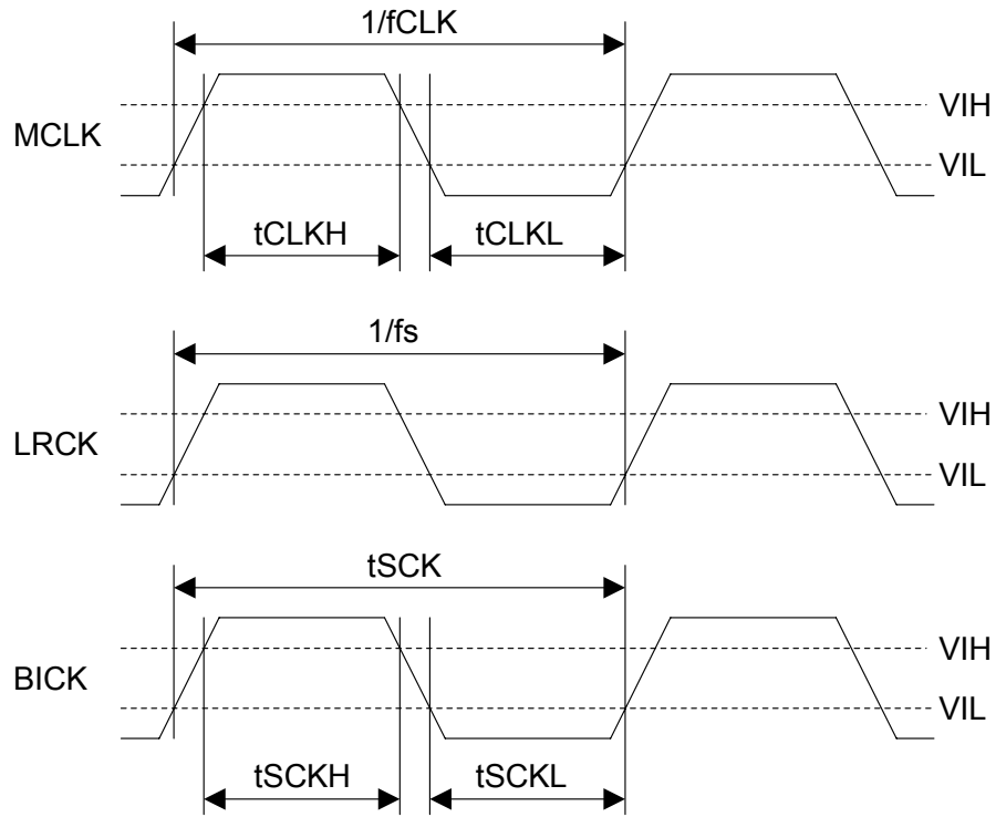
Figure 3. Clock Timing
