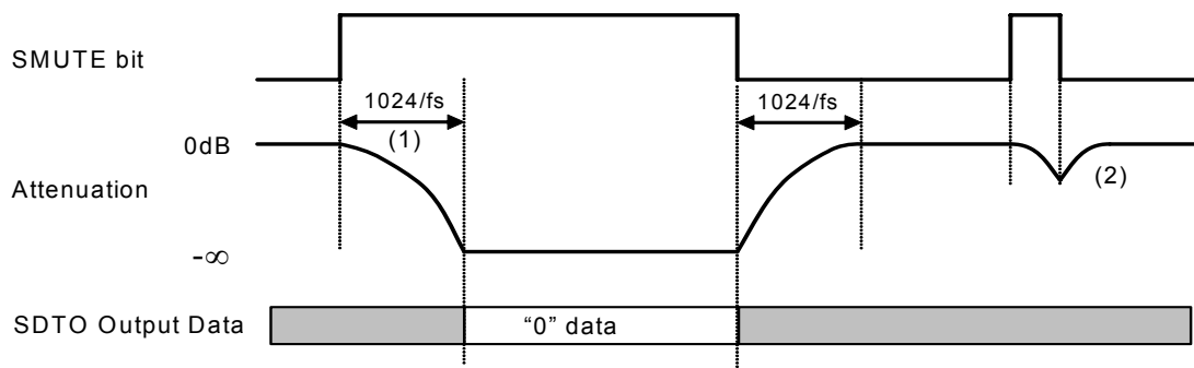
Figure 11. Soft Mute Function
