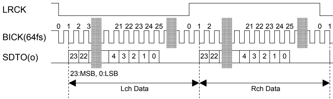
Figure 9. Mode 1 Timing
