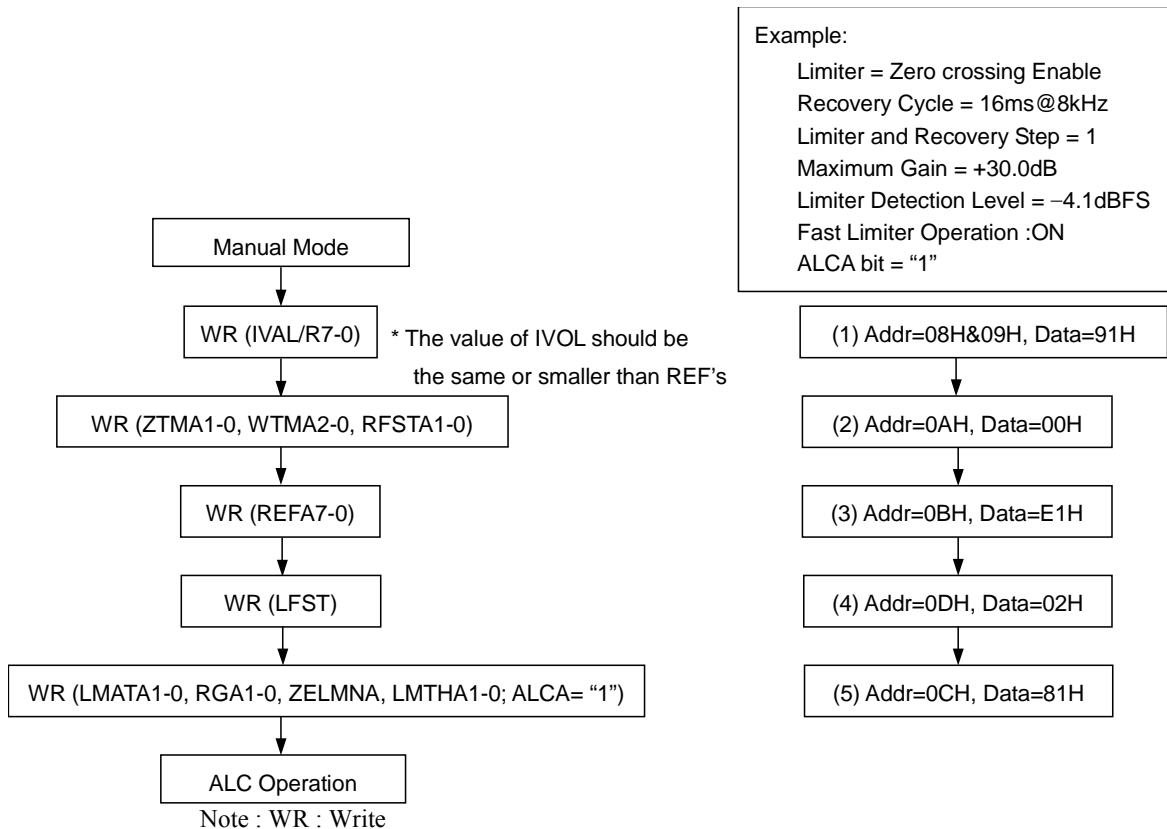
Figure 43. Registers set-up sequence at ALCA operation
