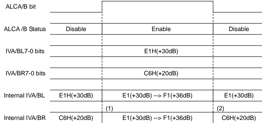
Figure 44. IVOL value during 2ch ALC operation
