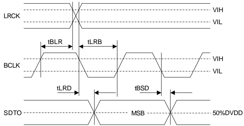
Figure 13. Audio Interface Timing (PLL/EXT Slave mode)
