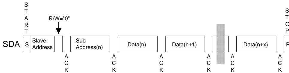
Figure 47. Data Transfer Sequence at the I 2 C-Bus Mode
