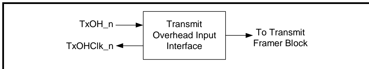
FIGURE 107. BLOCK DIAGRAM OF THE E1 TRANSMIT OVERHEAD INPUT INTERFACE OF XRT84L38
