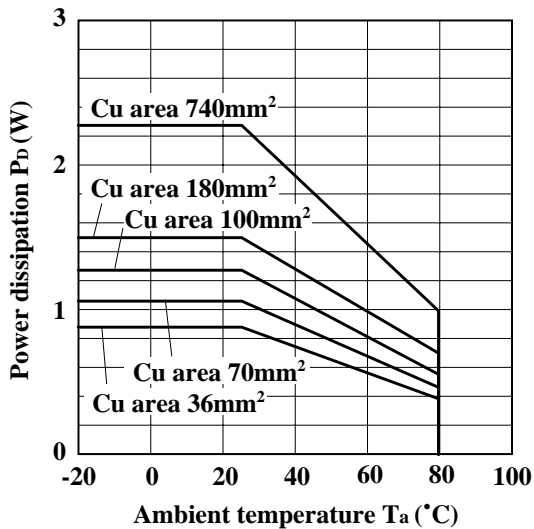
Fig.14 Power Dissipation vs. Ambient Temperature(Typical Value)
