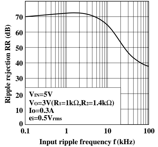
Fig.12 Ripple Rejection vs. Input Ripple Frequency
