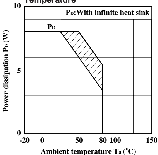
Fig.3 Power Dissipation vs. Ambient Temperature
