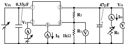
Fig.1 Test Circuit
