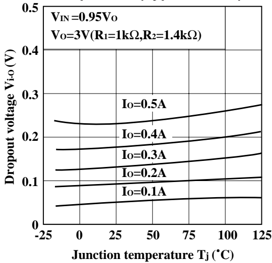
Fig.9 Dropout Voltage vs. Junction Temperature(Typical Value)
