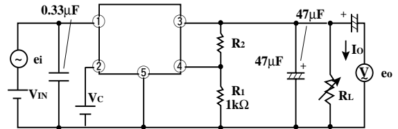
Fig.2 Test Circuit for Ripple Rejection
