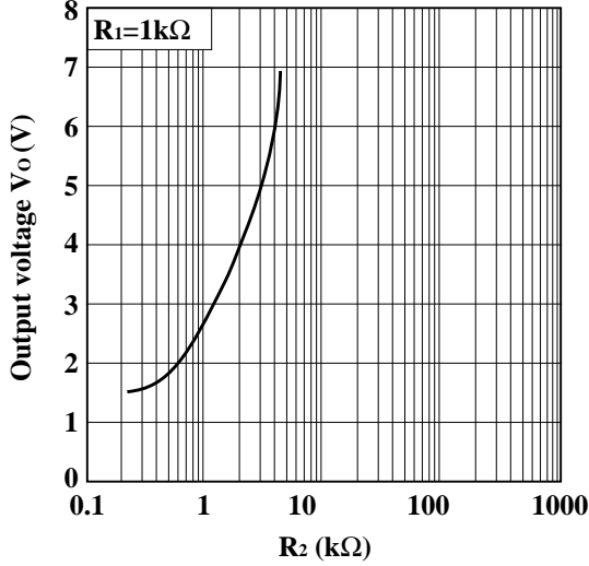
Fig.5 Output Voltage Adjustment Characteristics
