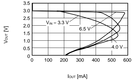
S-L2985B30 (Ta = 25°C)
