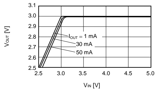
S-L2985B30 (Ta = 25°C)
