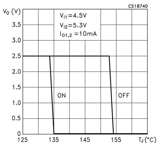
Figure 24: Thermal Protection vs V_{O1}
