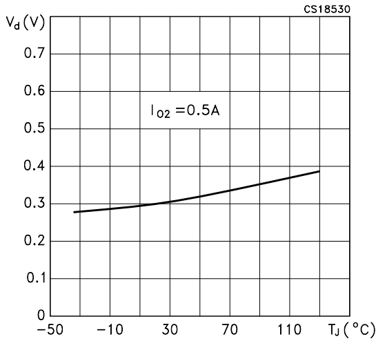
Figure 5: Dropout Voltage ( V_{O2} ) vs Temperature
