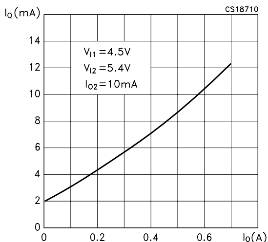
Figure 23: Quiescent Current ( V_{O2} ) vs Output Current
