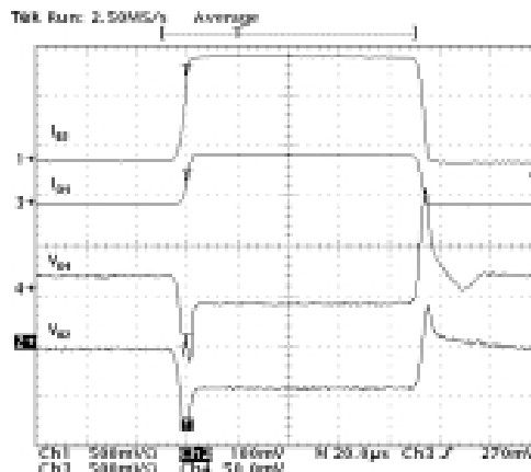
Figure 25: Load Transient
