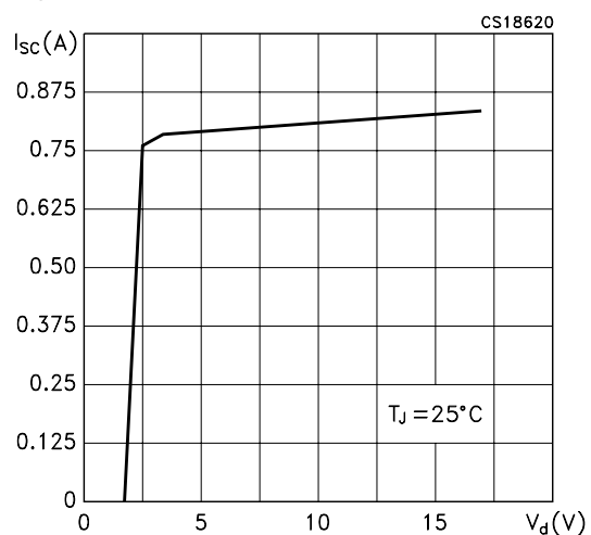
Figure 12: Short Circuit Current ( V_{O1} ) vs Drop Voltage
