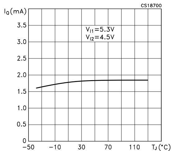
Figure 21: Total Supply Current vs Temperature
