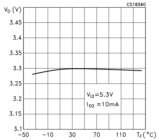
Figure 8: Line Regulation ( V_{O1} ) vs Temperature
