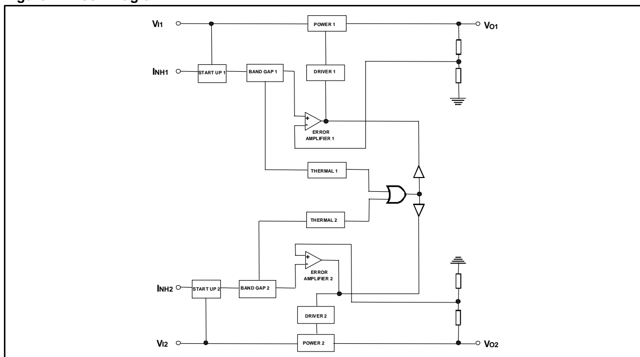
Figure 1: Block Diagram
