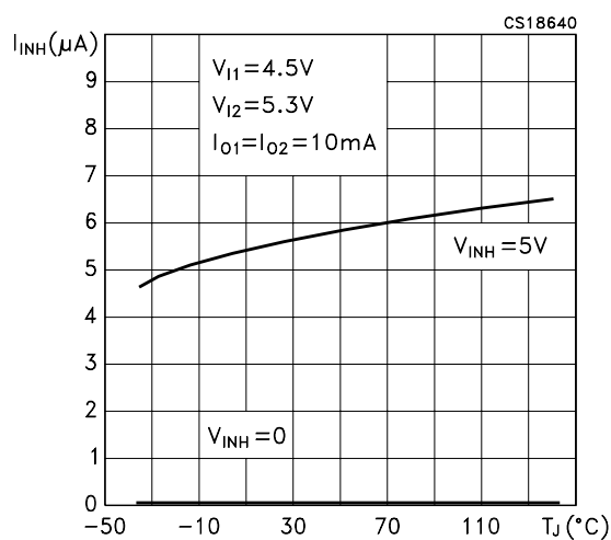
Figure 15: One Channel Inhibit Current vs Temperature
