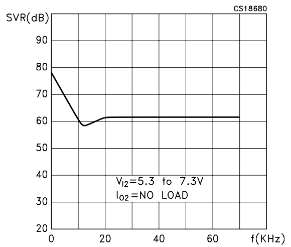
Figure 19: Supply Voltage Rejection ( V_{O2} ) vs Frequency
