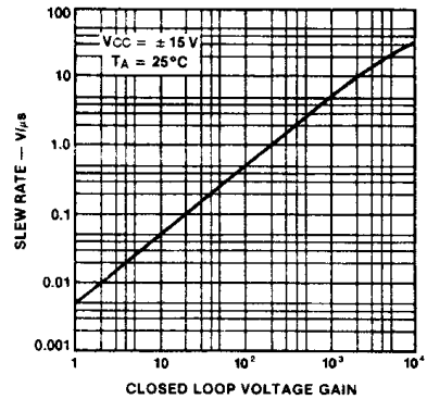
Slew Rate vs Closed Loop Gain
