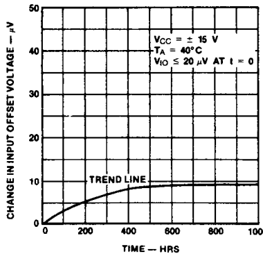
Input Offset Voltage Drift vs Time
