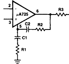
Frequency Compensation Circuit
