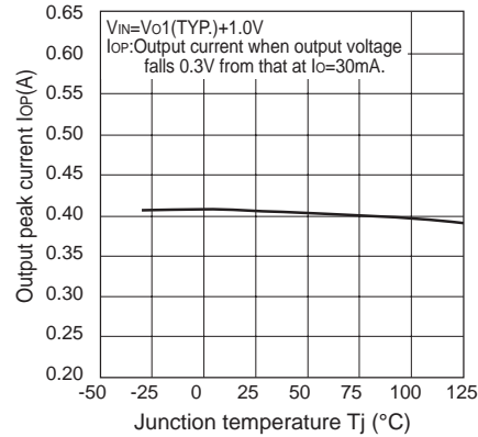
Fig.13 Output Peak Current vs. Junction Temperature(Typical Value)
