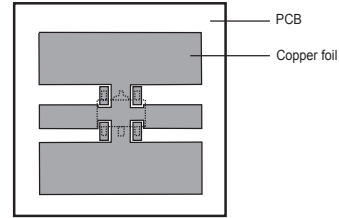
Mounting PCB
