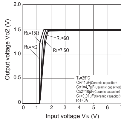
Fig.7 Output Voltage(Vo2) vs. Input Voltage (PQ2L3152MSPQ)(Typical Value)
