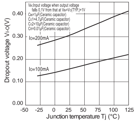
Fig.9 Dropout Voltage vs. Junction Temperature (PQ2L3252MSPQ)(Typical Value)
