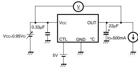
Fig.3 Measurement circuit for minimum I/O voltage differential
