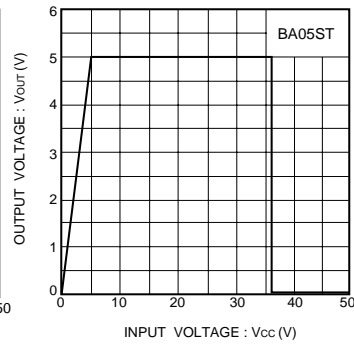
Fig. 9 Current limit characteristics
