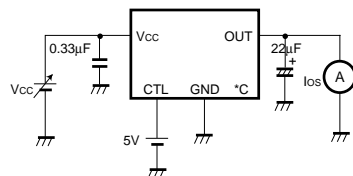
Fig.5 Measurement circuit for output short-circuit current
