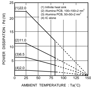
Fig. 7 Thermal derating curves (TO220FP-5)
