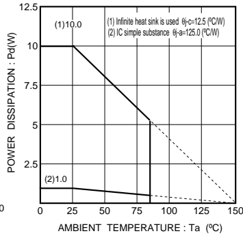
Fig. 8 Thermal derating curves (TO252-5)
