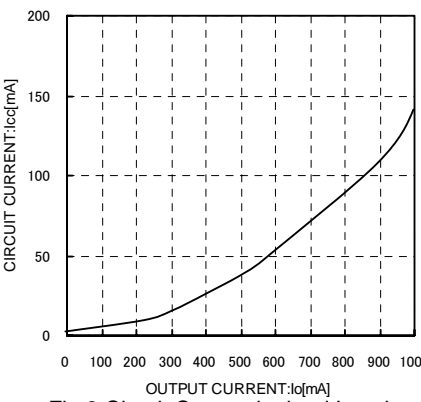
Fig.8 Circuit Current by load Level ( I_{oUT}=0mA \rightarrow 1A )
