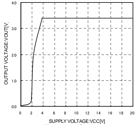
Fig.3 Input Stability
