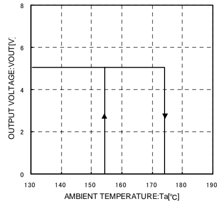
Fig.24 Thermal Shutdown Circuit Characteristics
