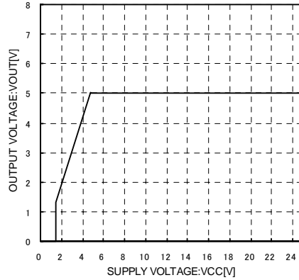
Fig.14 Input Stability
