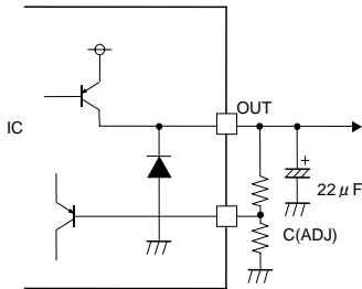
Fig.33: Output equivalent circuit
