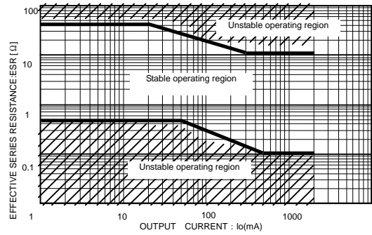
Fig.35: I_o vs. ESR characteristics (BA□□DD0, 22\ \mu\text{F} )
