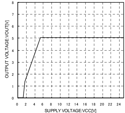
Fig.15 Input Stability ( I_o=2A )
