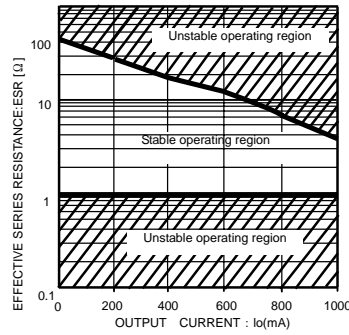
Fig.34: I_o vs. ESR characteristics (BA□□CC0, 22\ \mu\text{F} )
