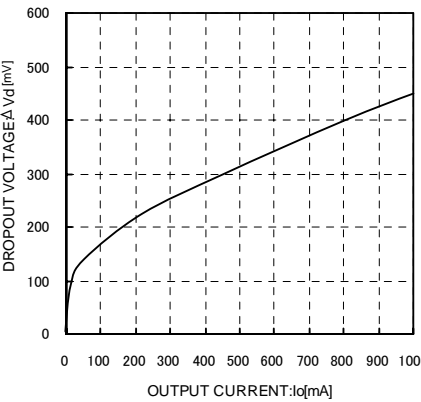
Fig.5 Input/Output Voltage Difference I_o-\Delta V_d Characteristics ( V_{CC}=2.95V )
