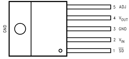
Top View TO220-5 Package Bent, Staggered Leads
