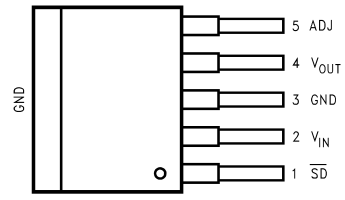
Top View TO263-5 Package
