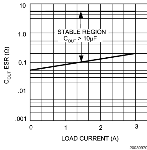
FIGURE 1. ESR Curve for C_{\text{OUT}} (with 10\mu\text{F} Tantalum Input Capacitor)
