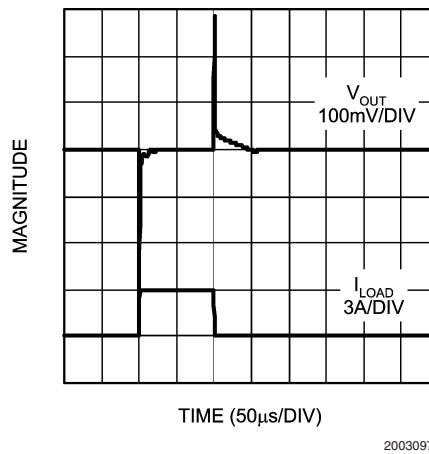
Load Transient Response C_{IN} = C_{OUT} = 10\mu\text{F} , TANTALUM
