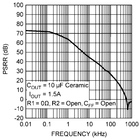
PSRR, I_{OUT} = 1.5A V_{OUT} = V_{ADJ} , C_{OUT} = 10 \mu F Ceramic
