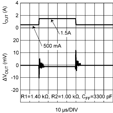
Load Transient, 500 mA to 1.5A V_{OUT} = 1.20V , C_{OUT} = 10 \mu F Ceramic
