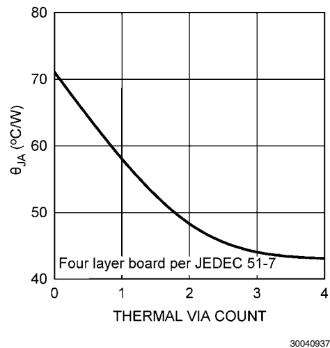
FIGURE 3. \theta_{JA} vs Thermal Via Count for the PSOP-8 Package on 2-Layer PCB with Copper Area on Bottom-Side
