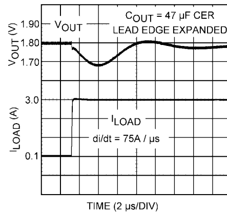
FIGURE 8. 47 \mu\text{F} Ceramic Output Capacitor
