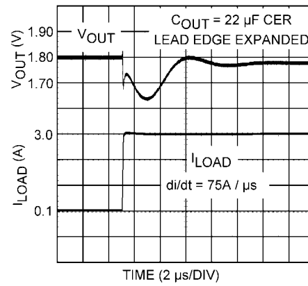
FIGURE 7. 22 \mu\text{F} Ceramic Output Capacitor
