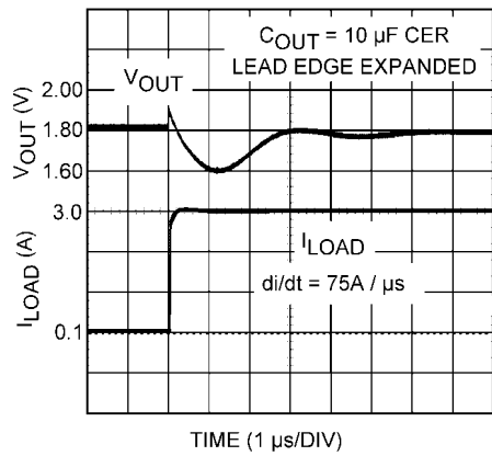
FIGURE 6. Rising Edge, 10 \mu\text{F} Ceramic, 75A/ \mu\text{s} di/dt
