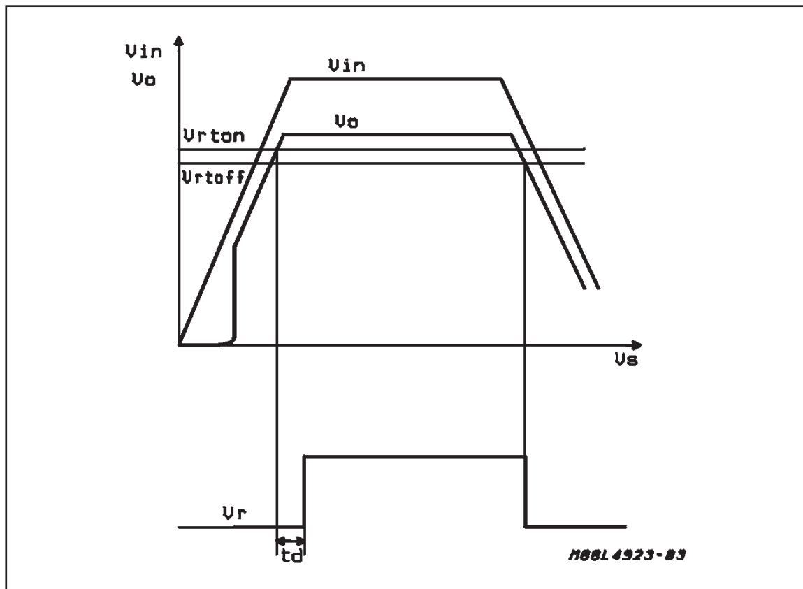
Figure 2 : Typical Reset Output Waveform.
