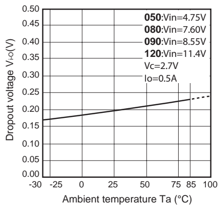
Fig.25 Dropout Voltage vs. Ambient Temperature (PQxxxRDA1SZH)
