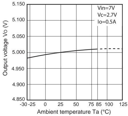
Fig.21 Output Voltage vs. Ambient Temperature (PQ050RDA1SZH)
