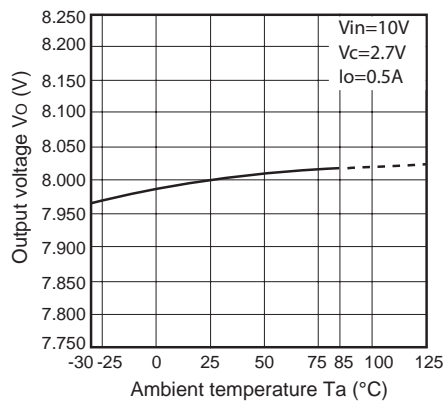
Fig.22 Output Voltage vs. Ambient Temperature (PQ080RDA1SZH)
