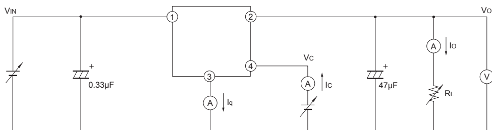
Fig.1 Test Circuit
