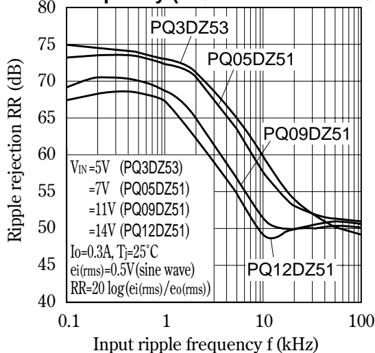
Fig.37 Ripple Rejection vs. Input Ripple Frequency (PQ05DZ51series/PQ3DZ53)
