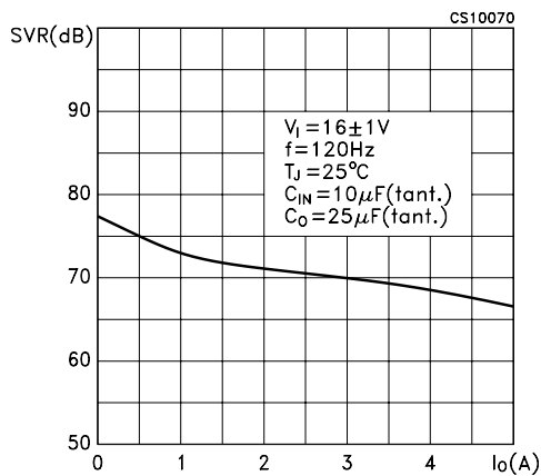
Figure 15 : Supply Voltage Rejection vs Output Current
