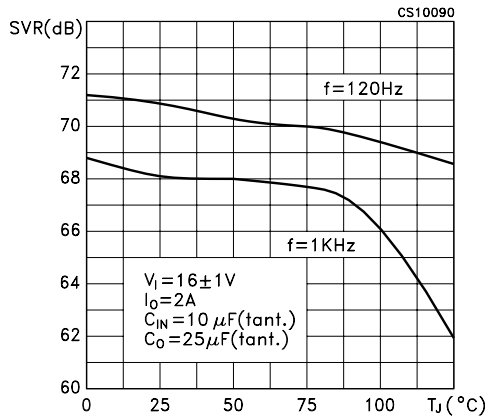
Figure 20 : Supply Voltage Rejection vs Temperature
