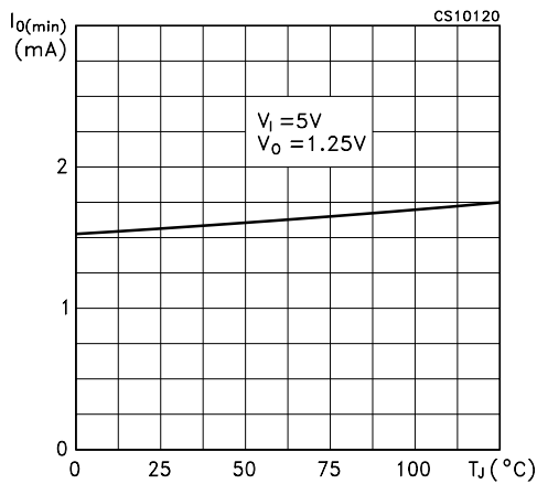
Figure 14 : Minimum Load Current vs Temperature
