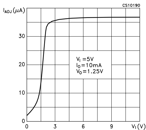
Figure 9 : Adjust Pin Current vs Input Voltage
