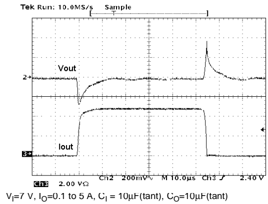
Figure 23 : Load Transient
