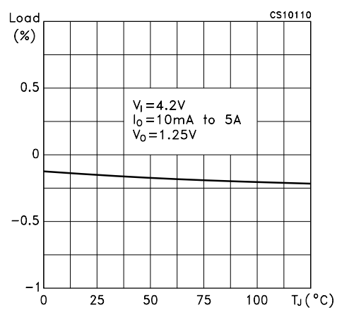
Figure 6 : Load Regulation vs Temperature
