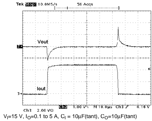
Figure 23 : Load Transient
