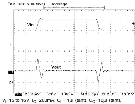
Figure 21 : Line Transient
