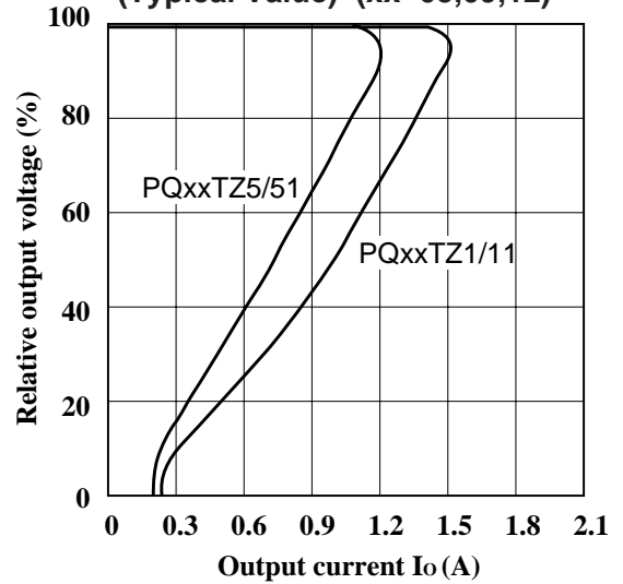
Fig.4 Overcurrent Protection Characteristics (Typical Value) (xx=05,09,12)
