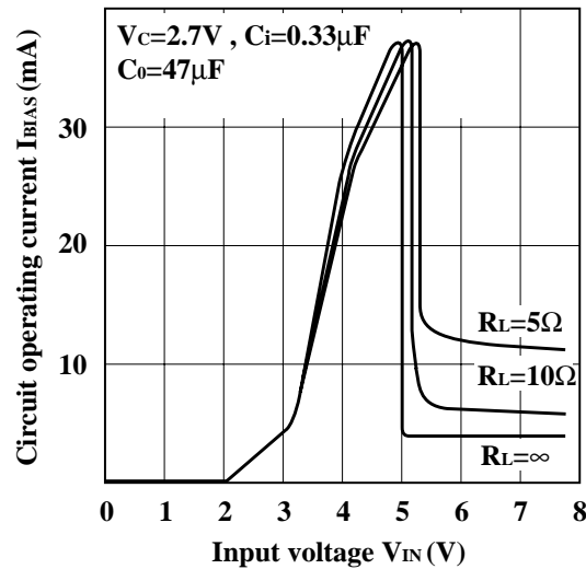
Fig.19 Circuit Operating Current vs. Input Voltage (PQ05TZ11)
