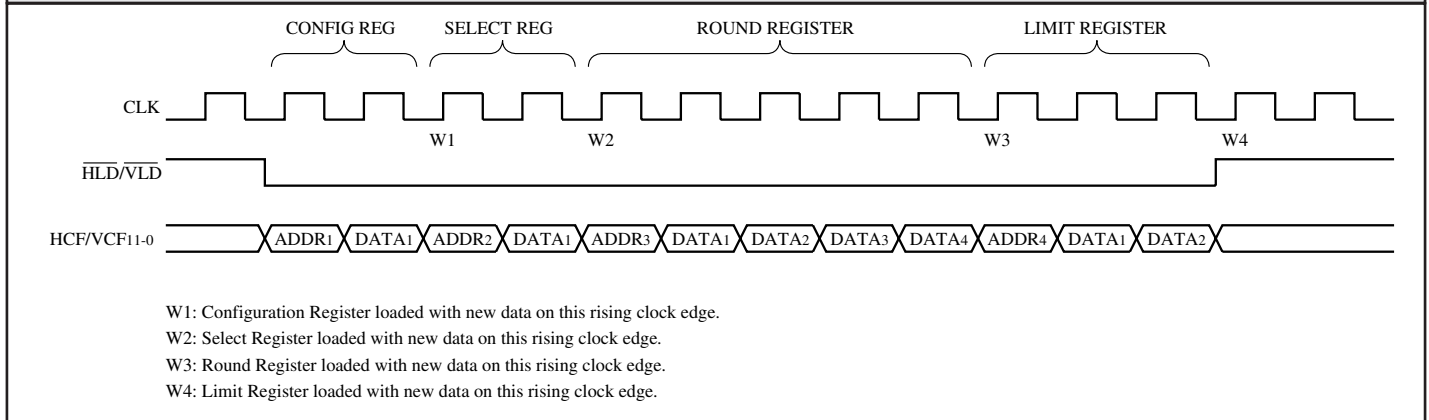
FIGURE 13. CONFIGURATION/CONTROL REGISTER LOADING SEQUENCE
