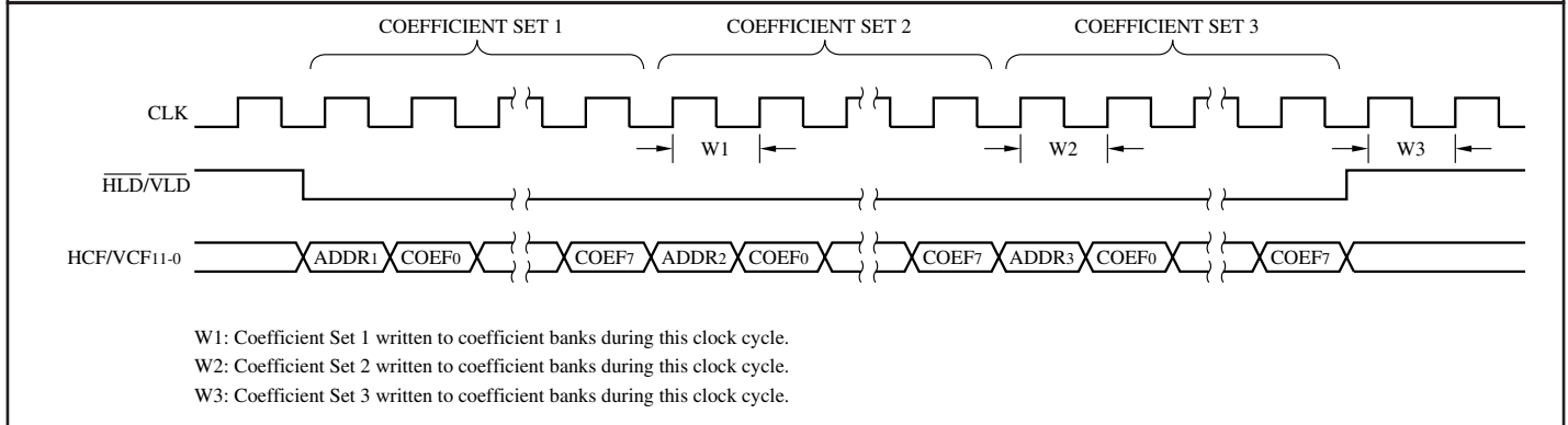
FIGURE 12. COEFFICIENT BANK LOADING SEQUENCE
