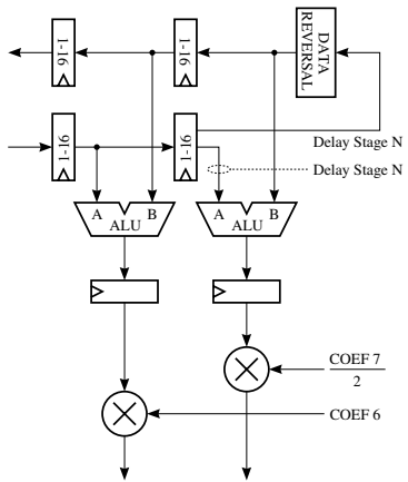
ODD-TAP MODE
