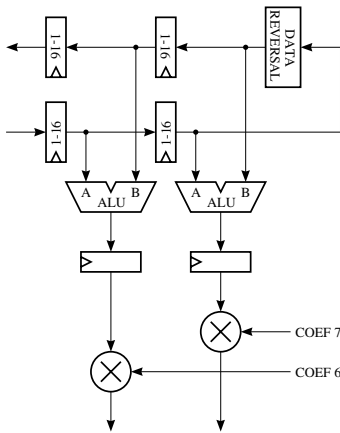
EVEN-TAP MODE
