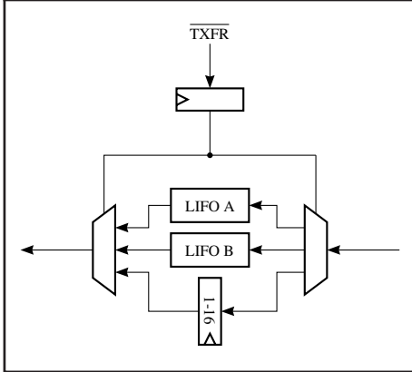
FIGURE 10. DATA REVERSAL
