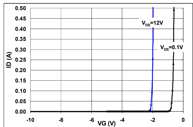
Figure 6 – Transfer Characteristic
