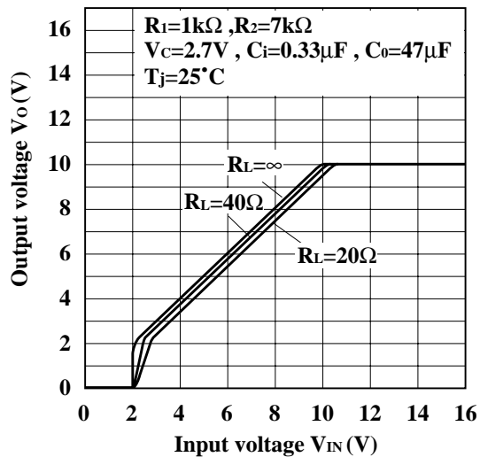
Fig.7 Output Voltage vs. Input Voltage (PQ20VZ51)
