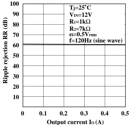
Fig.13 Ripple Rejection vs. Output Current (PQ20VZ51)
