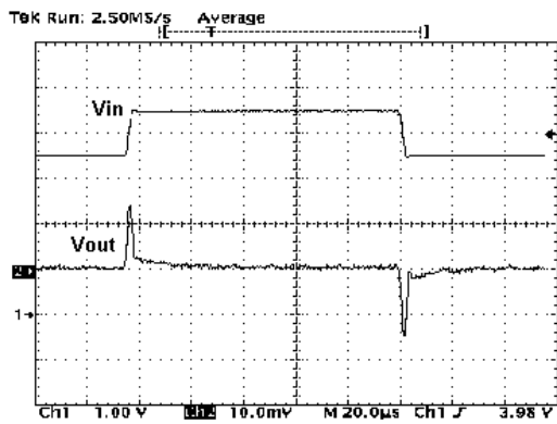
Figure 25 : Line Transient
