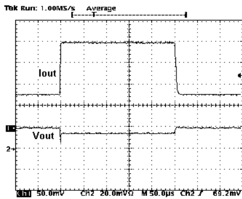
Figure 26 : Load Transient
