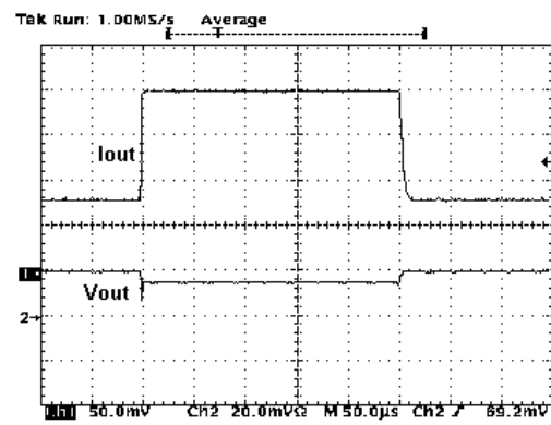
Figure 27 : Load Transient
