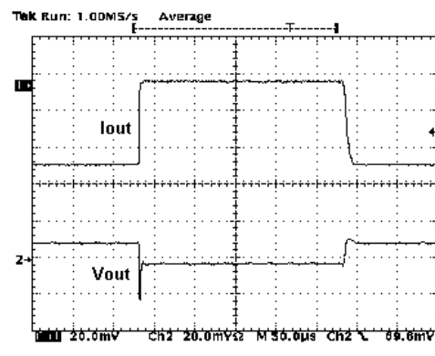
Figure 28 : Load Transient
