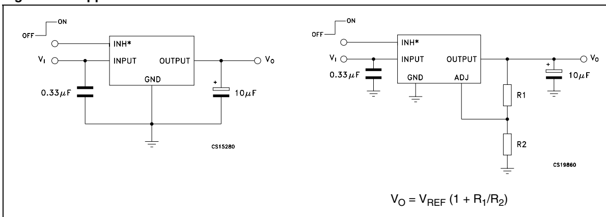
Figure 4. Application circuit
