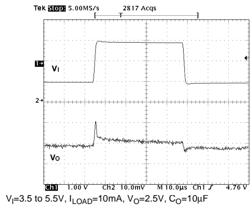
Figure 12 : Line Transient
