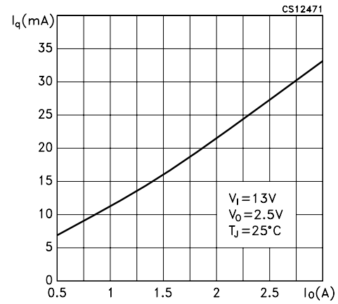
Figure 5 : Quiescent Current vs Output Current
