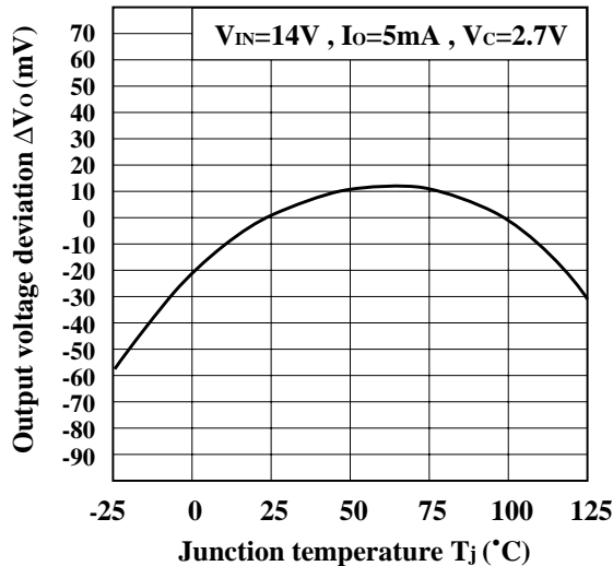
Fig.7 Output Voltage Deviation vs. Junction Temperature (PQ12TZ51/11)
