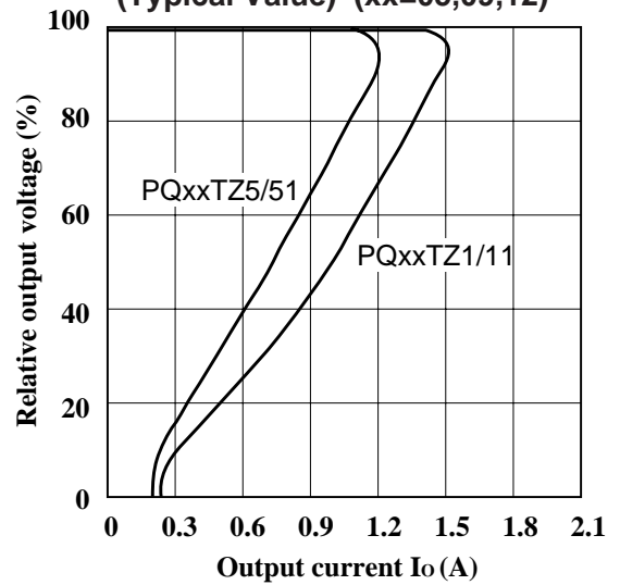
Fig.4 Overcurrent Protection Characteristics (Typical Value) (xx=05,09,12)
