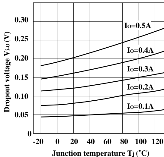
Fig.14 Dropout Voltage vs. Junction Temperature (PQ05TZ51/PQ09TZ51/PQ12TZ51)
