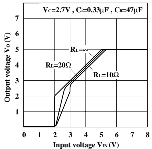
Fig.8 Output Voltage vs. Input Voltage (PQ05TZ51)
