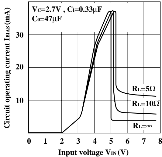
Fig.19 Circuit Operating Current vs. Input Voltage (PQ05TZ11)
