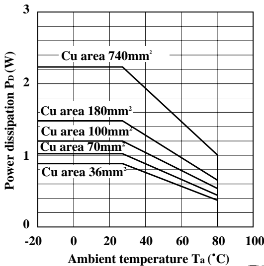
Fig.31 Power Dissipation vs. Ambient Temperature (Typical Value)
