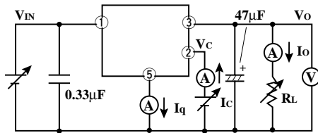
Fig.1 Test Circuit
