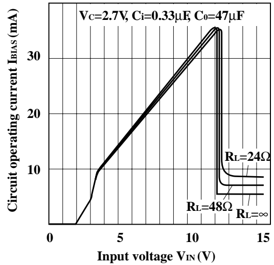
Fig.20 Circuit Operating Current vs. Input Voltage (PQ09TZ11)
