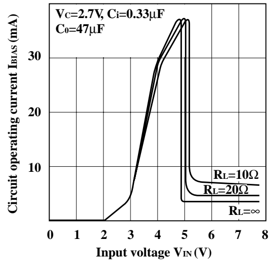
Fig.18 Circuit Operating Current vs. Input Voltage (PQ12TZ51)
