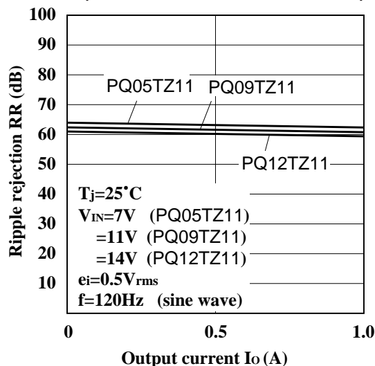
Fig.26 Ripple Rejection vs. Output Current (PQ05TZ11/PQ09TZ11/PQ12TZ11)
