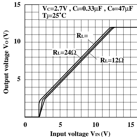
Fig.13 Output Voltage vs. Input Voltage (PQ12TZ11)
