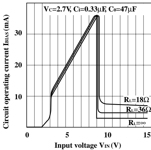
Fig.19 Circuit Operating Current vs. Input Voltage (PQ05TZ11)
