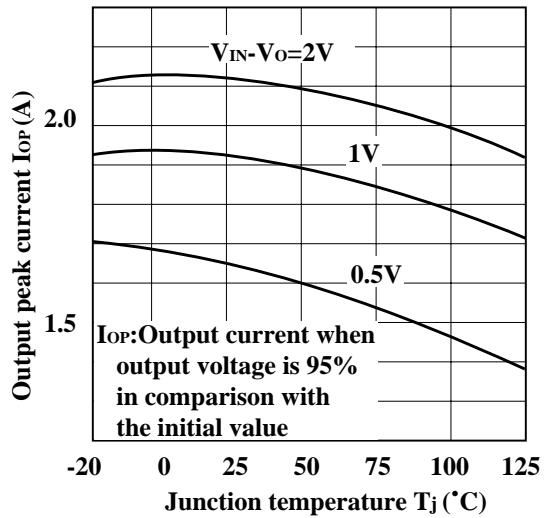
Fig.30 Output Peak Current vs. Junction Temperature (PQ05TZ11/PQ09TZ11/PQ12TZ11)
