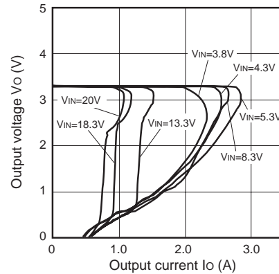
Fig.4 Overcurrent Protection Characteristics (PQ033RDA2SZH)
