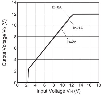
Fig.11 Output Voltage vs. Input Voltage (PQ120RDA2SZH)
