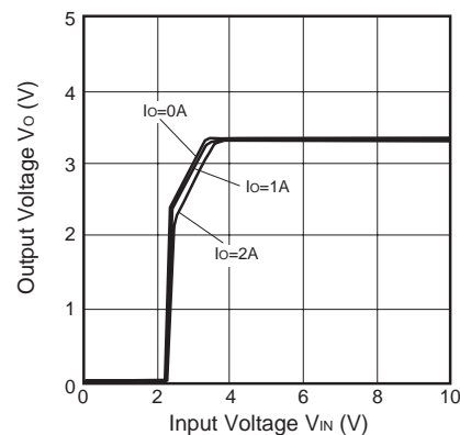
Fig.8 Output Voltage vs. Input Voltage (PQ033RDA2SZH)
