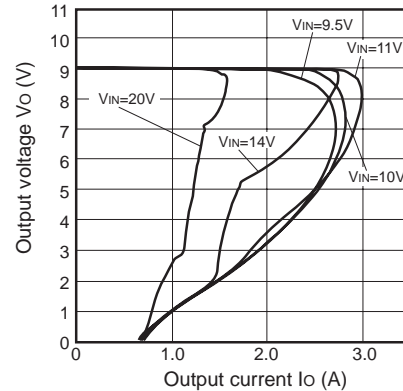
Fig.6 Overcurrent Protection Characteristics (PQ090RDA2SZH)
