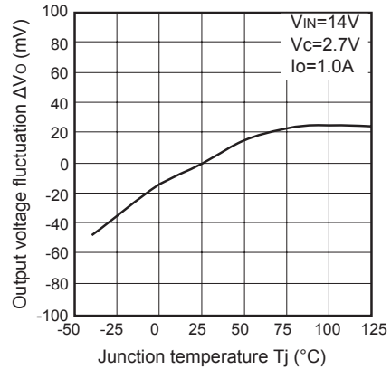
Fig.20 Output Voltage Fluctuation vs. Junction Temperature (PQ120RDA2SZH)
