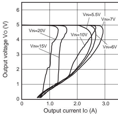
Fig.5 Overcurrent Protection Characteristics (PQ050RDA2SZH)
