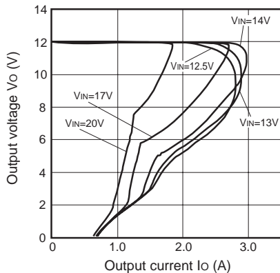
Fig.7 Overcurrent Protection Characteristics (PQ120RDA2SZH)
