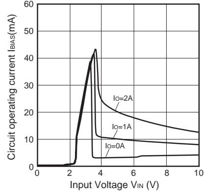
Fig.12 Circuit Operating Current vs. Input Voltage (PQ033RDA2SZH)
