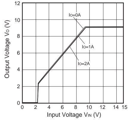
Fig.10 Output Voltage vs. Input Voltage (PQ090RDA2SZH)
