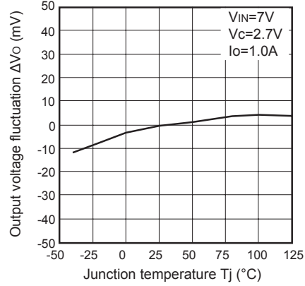
Fig.18 Output Voltage Fluctuation vs. Junction Temperature (PQ050RDA2SZH)
