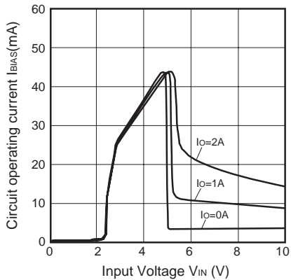
Fig.13 Circuit Operating Current vs. Input Voltage (PQ050RDA2SZH)
