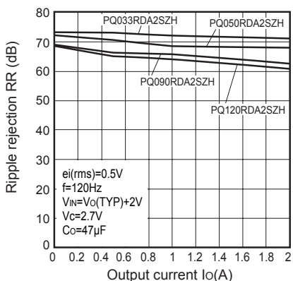
Fig.25 Ripple Rejection vs. Output Current (PQxxxRDA2SZH)
