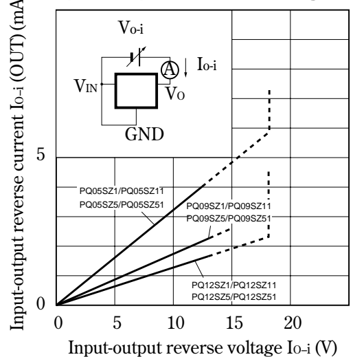
Fig.26 Input-Output Reverse Current vs. Input-Output Reverse Voltage
