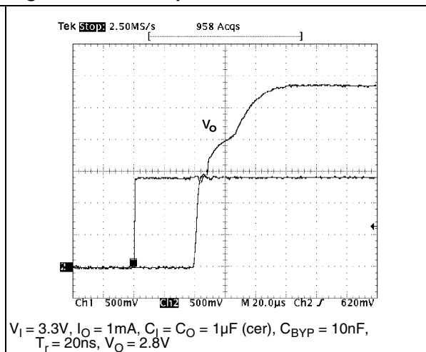
Figure 21. Start-Up
