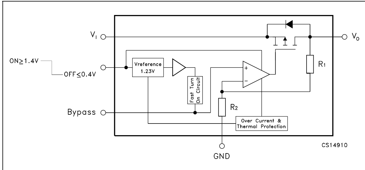
Figure 1. Schematic diagram
