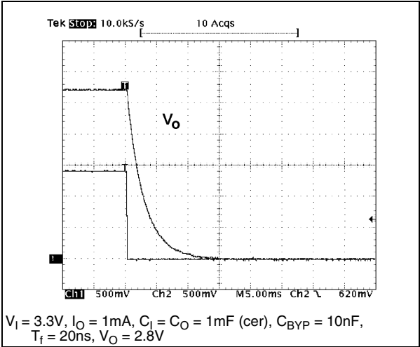
Figure 22. Turn-Off
