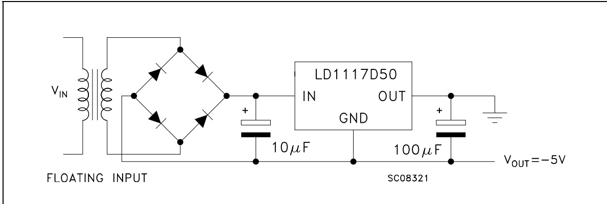
Figure 5. Negative supply
