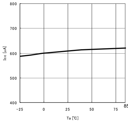
Fig.8 Ta-Icc
