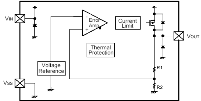
XC6701D Series (SOT-89, SOT-223, TO-252)
