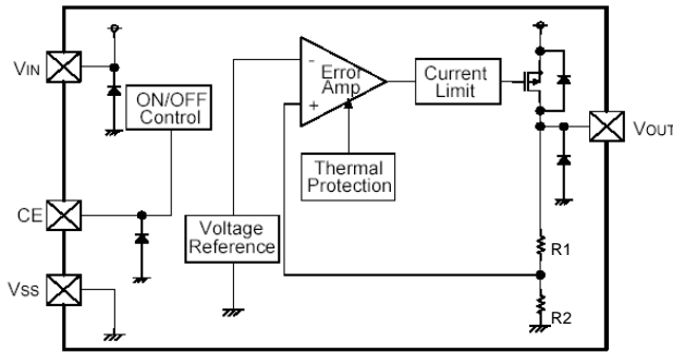
XC6701B Series (SOT-25, SOT-89-5, USP-6C)
