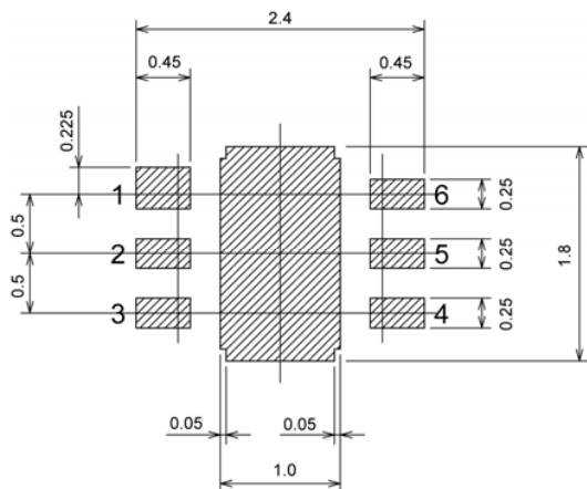
USP-6C Reference Pattern Layout
