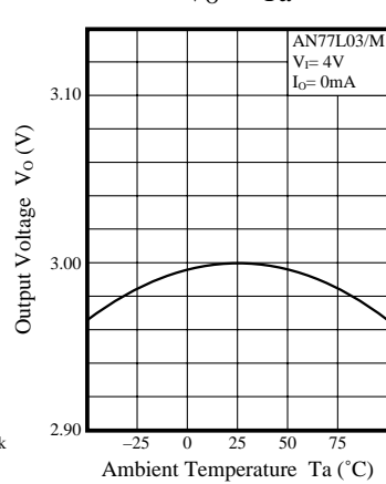
Output Voltage Temperature Characteristics V_O - T_a
