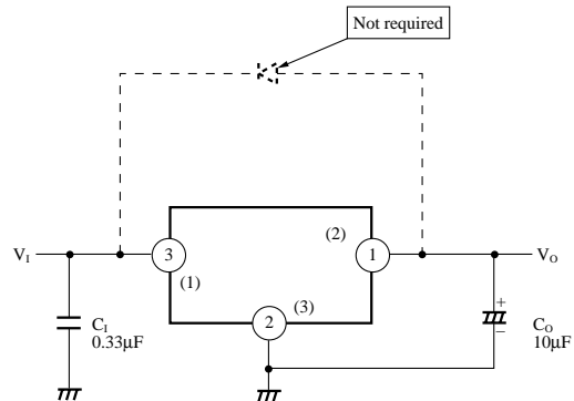
Pin number in \circ is for the AN77L00M series. Pin number in ( ) is for the AN77L00 series.
