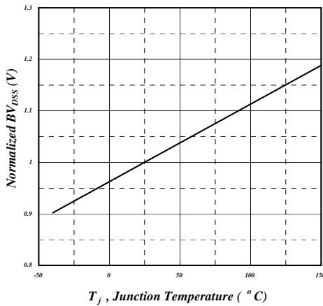
Fig 3. Normalized BV_{DSS} v.s. Junction Temperature
