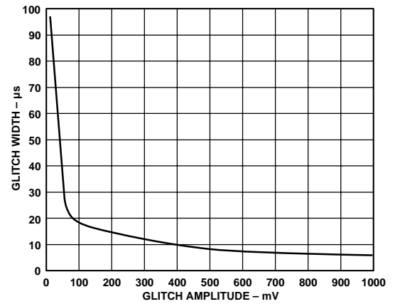
Figure 22. Glitch Immunity
