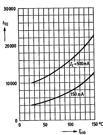
DC current gain h_{FE} = f(T_{amb})
