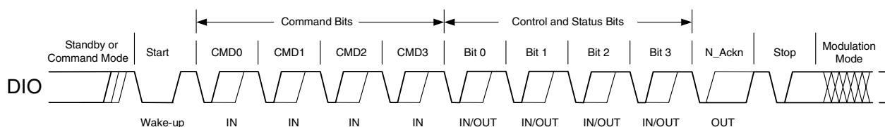
Figure 8. Control/Status Command Structure
