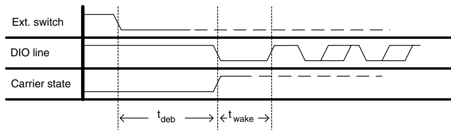
Figure 4. Wake-up by External Switch, Automatic Field Generation
