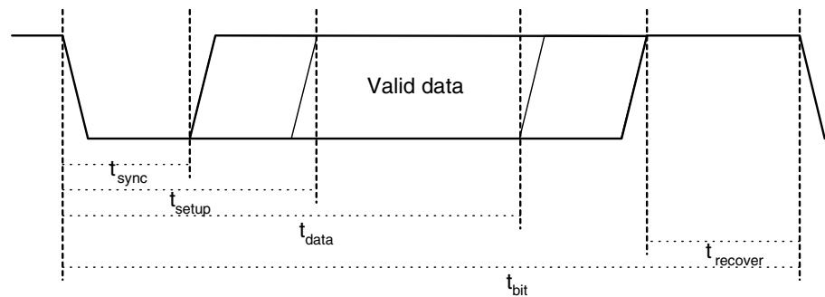
Figure 6. Structure of One Communication Bit
