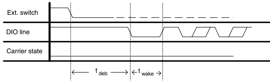
Figure 3. Wake-up by External Switch
