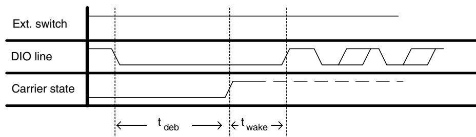
Figure 5. Wake-up by Connected Microcontroller, Automatic Field Generation
