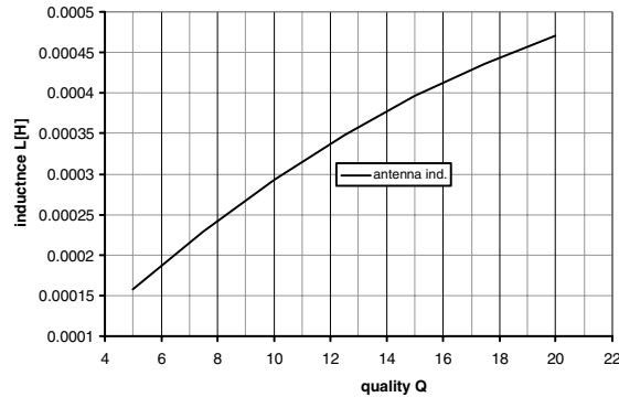
Figure 11. Antenna Coil Inductance versus Quality
