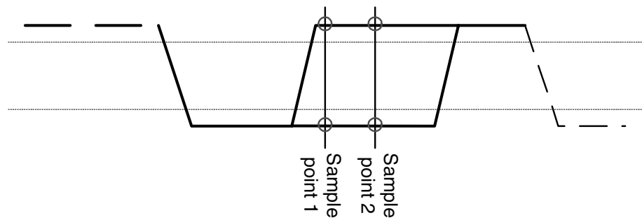
Figure 7. Data Consistency Check
