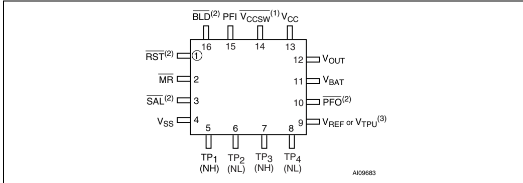
Figure 2. QFN16 connections
