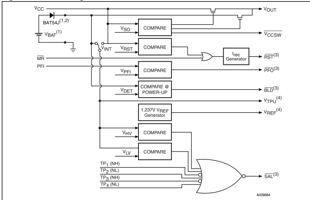
Figure 3. Block diagram
