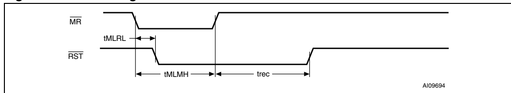
Figure 25. \overline{MR} timing waveform
