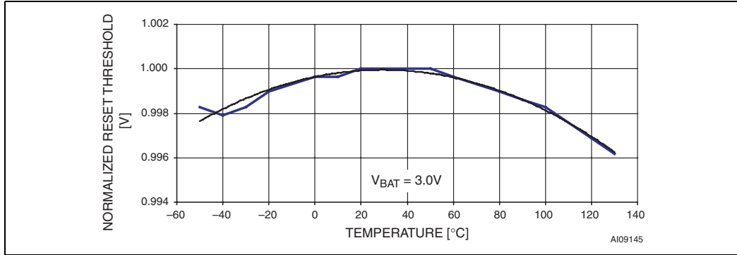
Figure 17. PFI to \overline{PFO} propagation delay vs. temperature
