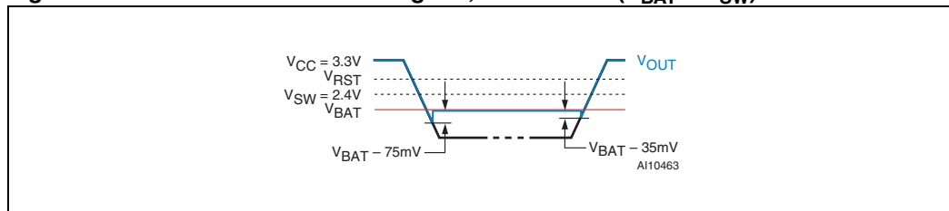
Figure 26. STM1403 switchover diagram, condition A ( V_{BAT} < V_{SW} )
