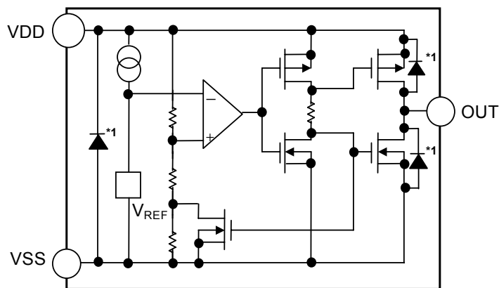
*1. Parasitic diode
