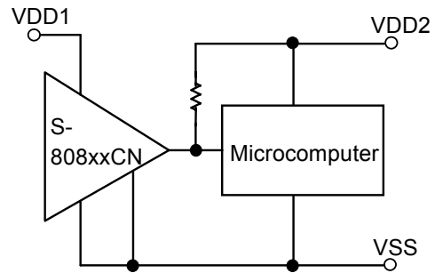
Figure 28 Reset Circuit Example (S-808xxCN)
