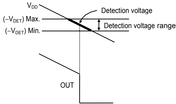
Figure 21 Detection Voltage (CMOS Output Products)
