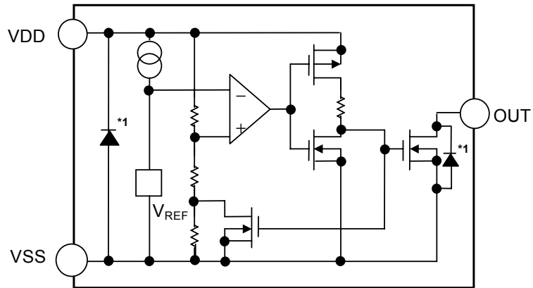
*1. Parasitic diode
