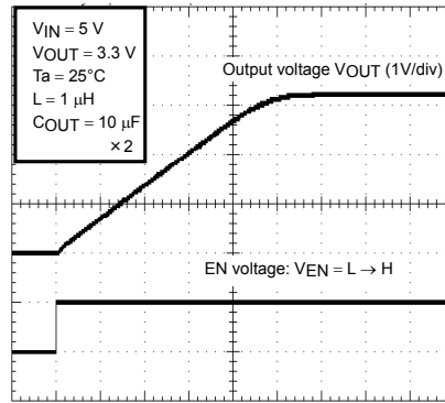
Startup Characteristics ( C_{SS} = 0.1\ \mu\text{F} )
