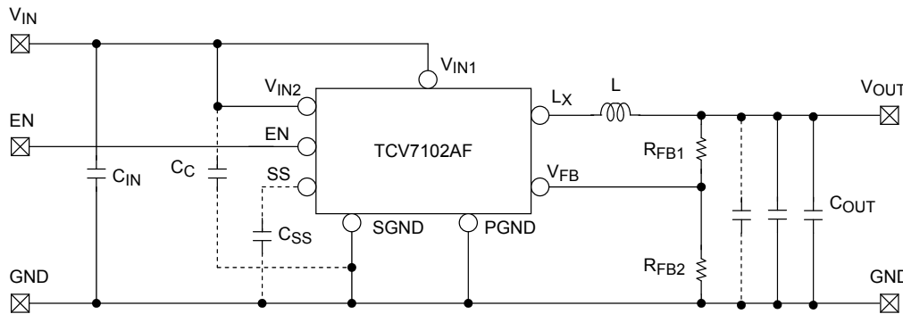
Figure 1 TCV7102AF Application Circuit Example
