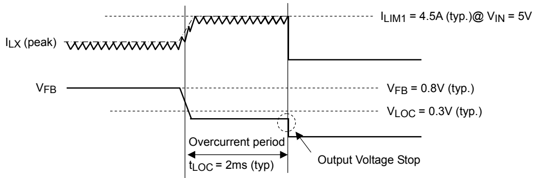
Figure 4 Overcurrent Operation
