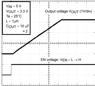
Startup Characteristics (Internal Soft-Start Time)
