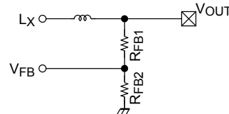
Figure 3 Output Voltage Setting Resistors
