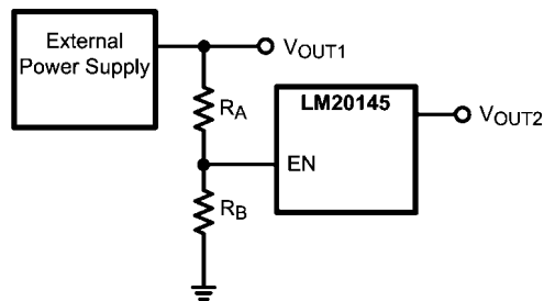
FIGURE 6. Sequencing LM20145 with Precision Enable
