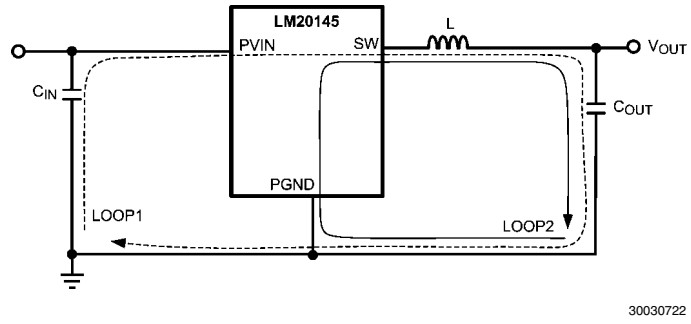
FIGURE 10. Schematic of LM20145 Highlighting Layout Sensitive Nodes
