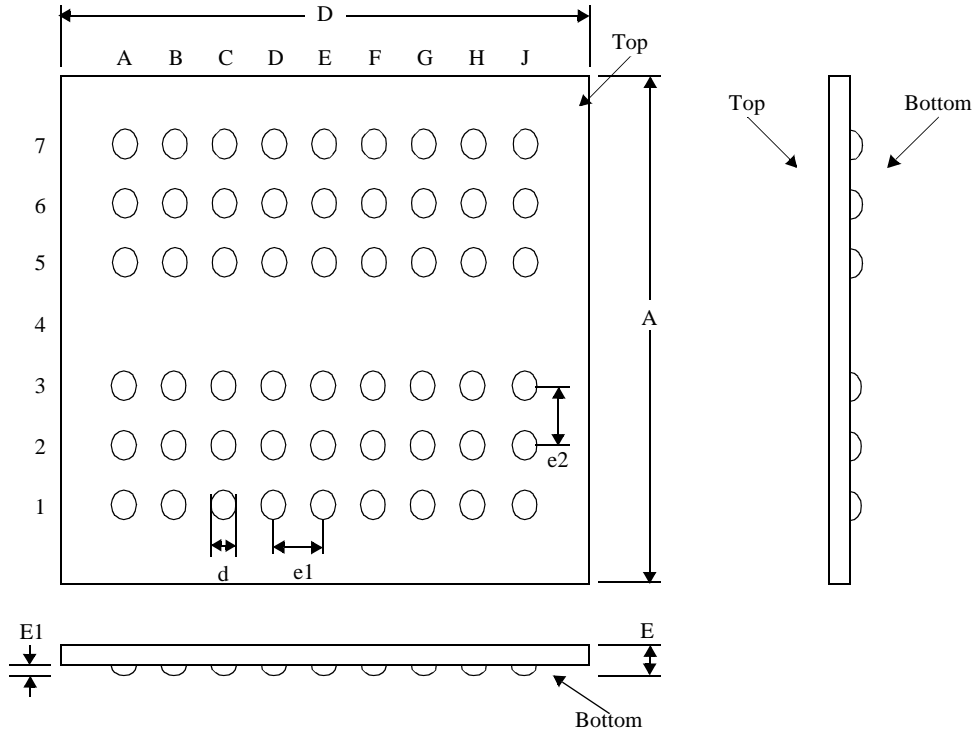
Figure 61: Center-Bonded uBGA Package
