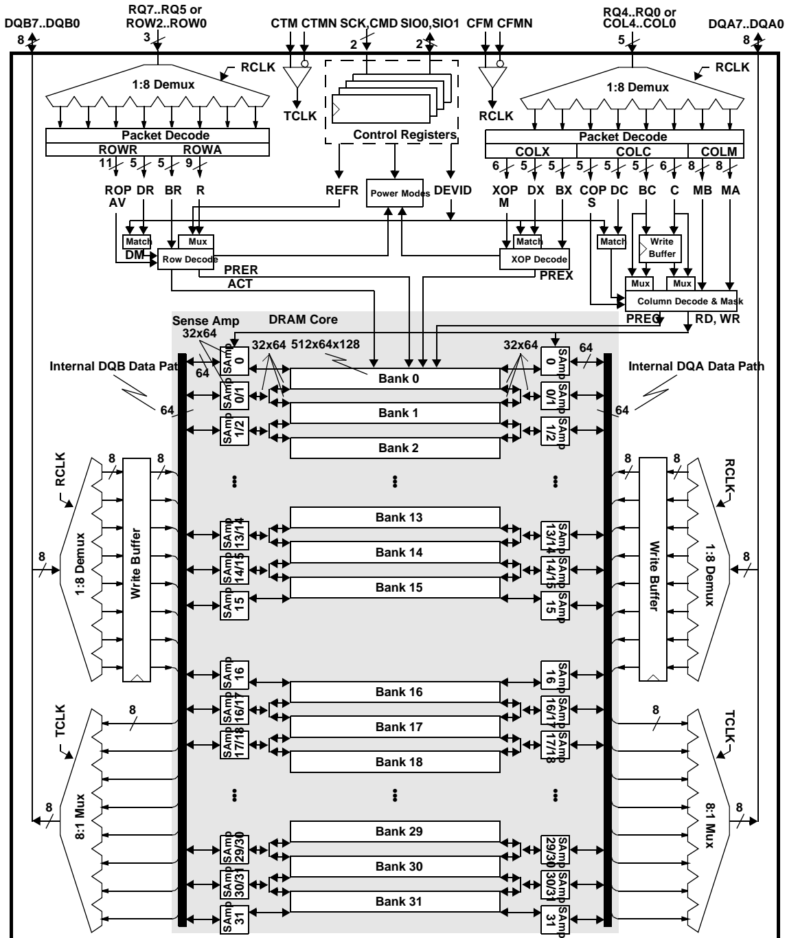
Figure 2: 128 Mbit Direct RDRAM Block Diagram
