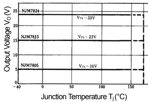
NJM7805/15/24 Output Voltage vs. Junction Temperature
