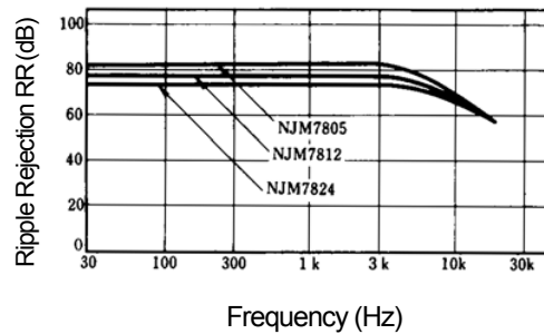
NJM7805/15/24 Ripple Rejection vs. Frequency
