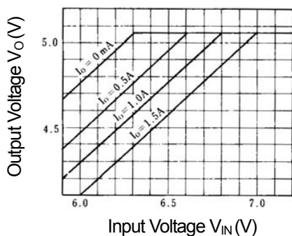
NJM7805 Dropout Characteristics ( T_j=25^\circ C )
