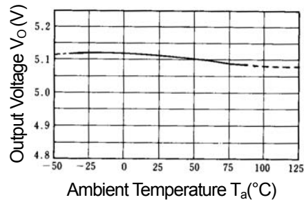
NJM7805 Output Voltage vs. Temperature
