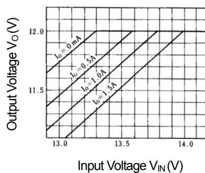
NJM7812 Dropout Characteristics ( T_j=25^\circ C )
