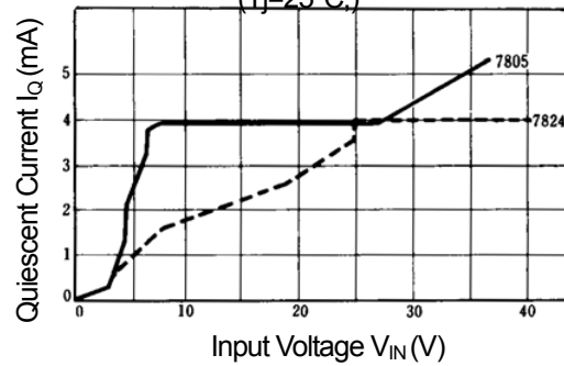
NJM7805/24 Quiescent Current vs. Input Voltage ( T_j=25^\circ\text{C} .)
