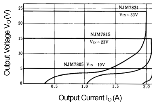
NJM7805/15/24 Load Characteristics ( T_j=25^\circ C )
