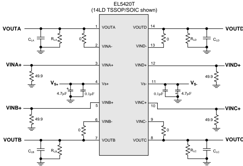
FIGURE 27. BASIC TEST CIRCUIT
