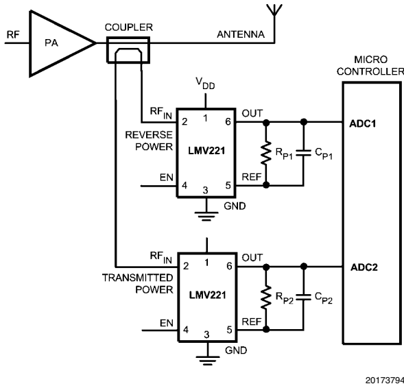
FIGURE 4. VSWR Application
