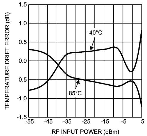
Mean Temperature Drift Error vs. RF Input Power at 2500 MHz
