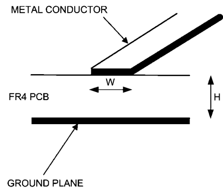
FIGURE 15. Microstrip Configuration
