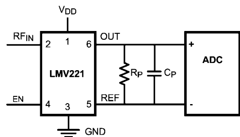
FIGURE 12. Single Ended and Differential Application
