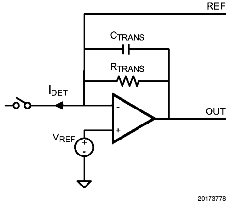
FIGURE 13. Output Stage of the LMV221
