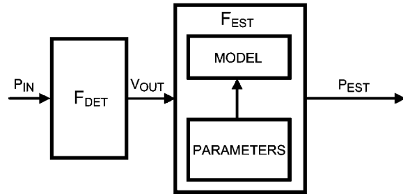
FIGURE 5. Generic Concept of a Power Measurement System
