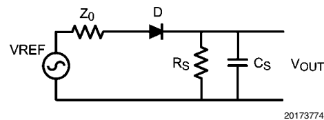
FIGURE 2. Diode Detector
