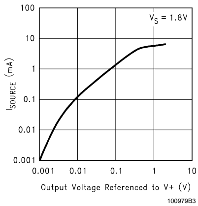
Sourcing Current vs. Output Voltage
