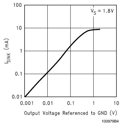
Sinking Current vs. Output Voltage
