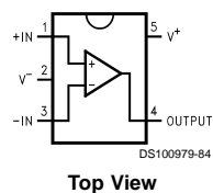
5-Pin SC70-5/SOT23-5
