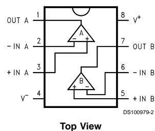
8-Pin MSOP/SOIC
