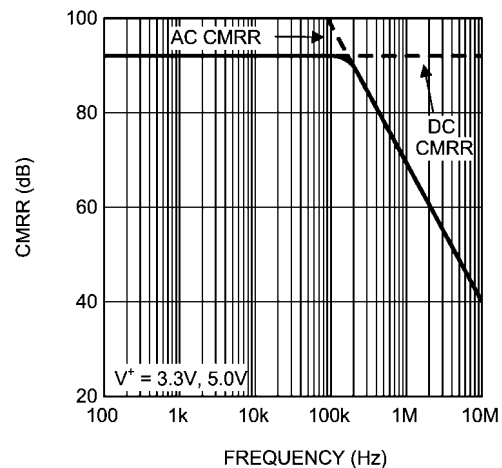
FIGURE 2. CMRR Curve
