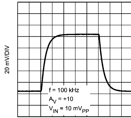
Small Signal Step Response with Gain = 10
