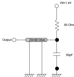
(Fig. 2) AC Output Load Circuit
