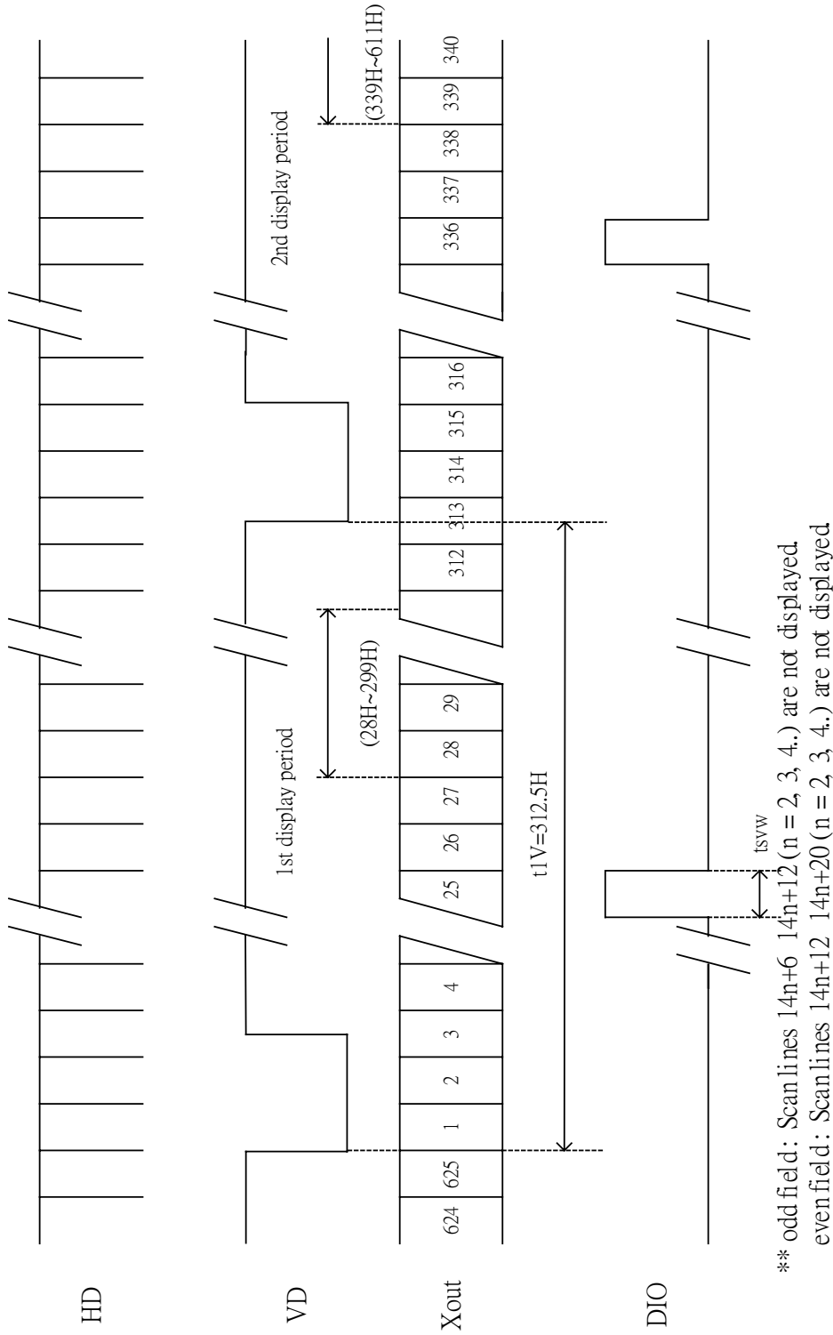
Fig. 8-1 Vertical Start Line for PAL
